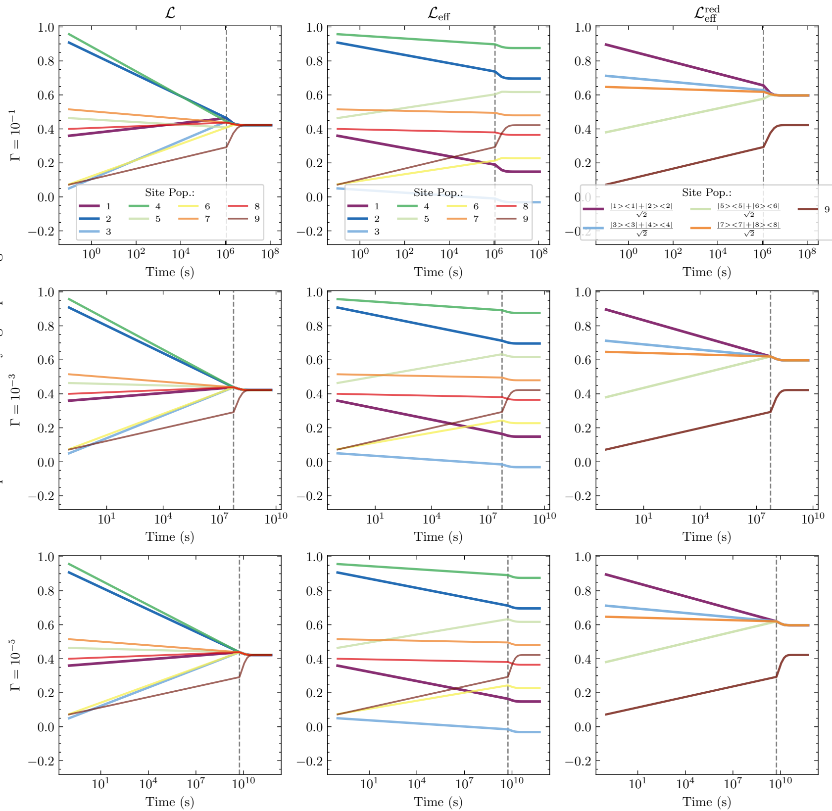
Time Evolution of Site Populations under \mathcal{L} , \mathcal{L}_{\text{eff}} , and \mathcal{L}_{\text{eff}}^{\text{red}} N=9 ; N_{\text{dimers}}=4 ; N_{\epsilon}=1 ; J = 10^{-1} ; \epsilon = 10^{-4} ; seed=491
